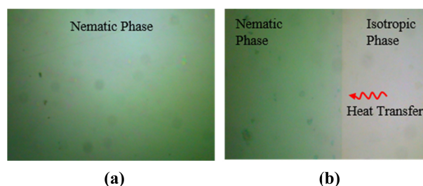
Fig. 3. POM images of 5CB during the nematic-isotropic phase transition (a) Nematic 5CB LC under thermal equilibrium, (b) 5CB LC under phase transition.
