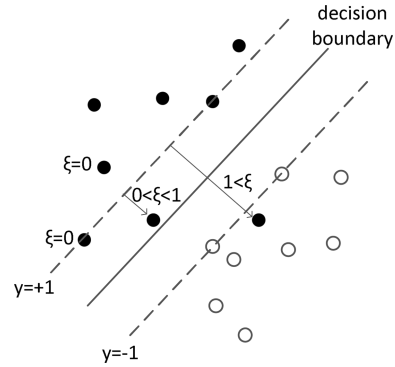
Fig. 2. SVM as a maximum margin classifier and slack variable \xi .
